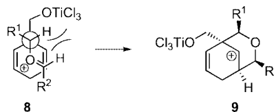
Scheme 7. Rationalisation of the stereochemical outcome.
