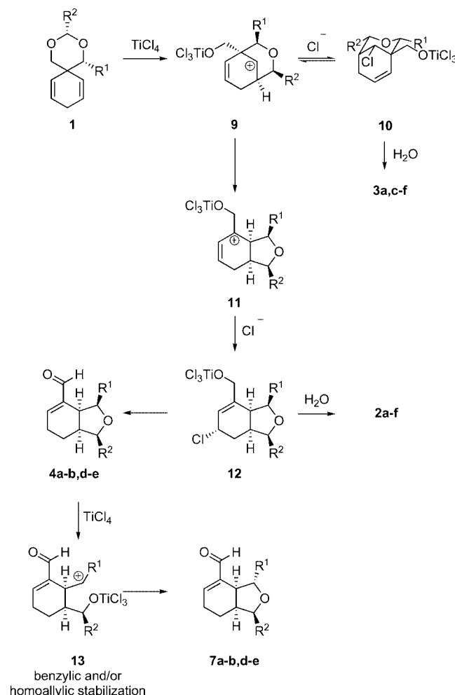
Scheme 8. Mechanistic summary.
